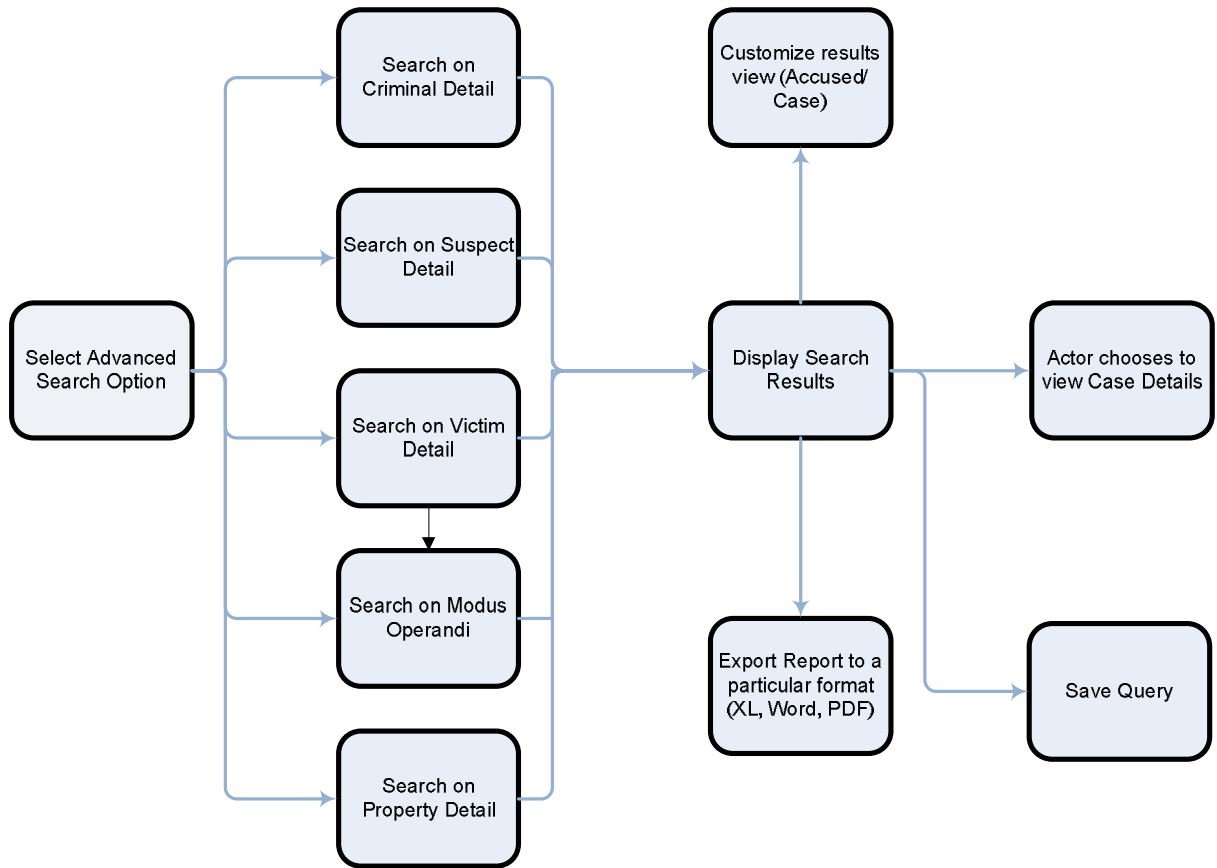
3.4.1 Diagram for Advanced Search
